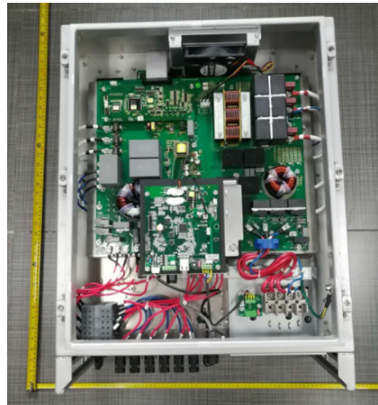
Figure 2 Converter Internal view
